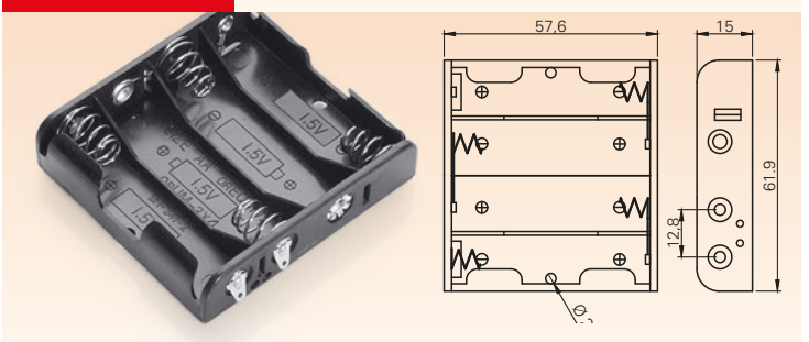
4 PCS AA SIZE BATTERY HOLDER
