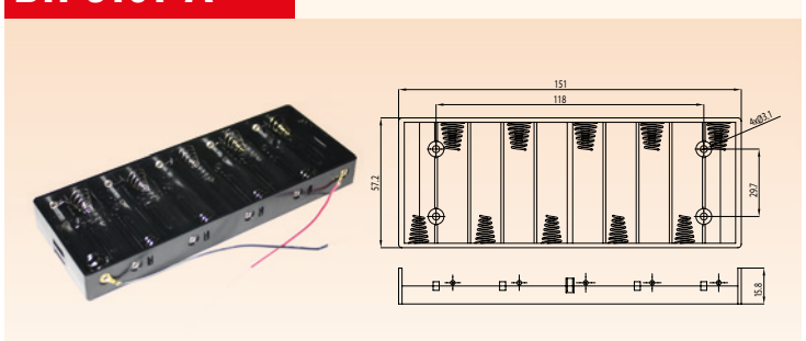
10 PCS AA SIZE BATTERY HOLDER
