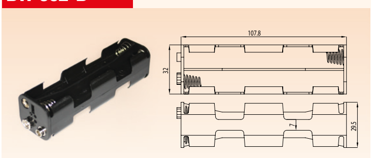
8 PCS AA SIZE BATTERY HOLDER
