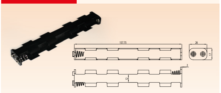
6 PCS AA SIZE BATTERY HOLDER
